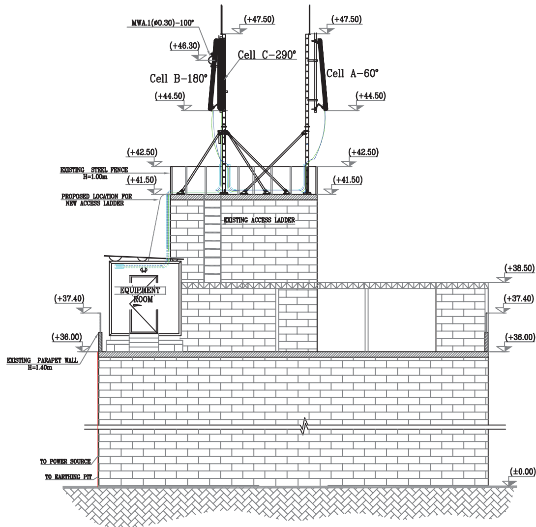
ELEVATION A SCALE 1:100
